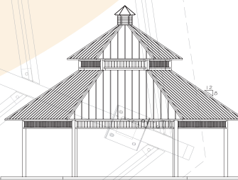
HEXAGON GAZEBO, Two-Tier: HS2G24, HS2G28, HS2G36
