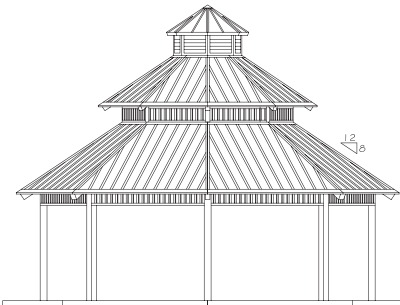
OCTAGON GAZEBO, Two-Tier: OS2G28
